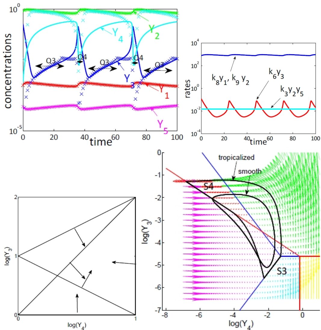
Fig. 1. (top left) Detection of slaved species by comparing traces to imposed traces: the species y_1, y_2, y_5 are slaved globally, the species y_3, y_4 are slaved on intervals Q_3, Q_4 , respectively. (top right) Comparison of monomials of the polynomial systems of quasi-steady state equations. (bottom left) Newton polygons and inner normals of the reduced two dimensional polynomial model. (bottom right) Phase portrait on logarithmic paper of the reduced two dimensional model. We represent the two tropical curves (the tripods graphs, a red and a blue one), the modes (smooth vector fields within domains bordered by tropical curves tentacles), the smooth and tropicalized limit cycles. The tropicalized cycle contains two sliding modes S_3, S_4 corresponding to the intervals Q_3, Q_4 on which y_3, y_4 are quasi-stationary, respectively.
